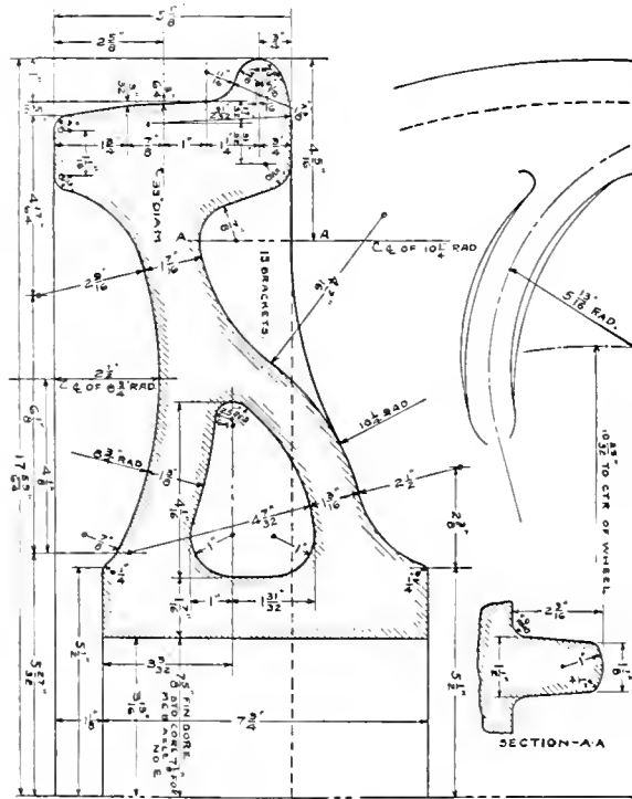
Fig. 3—Cast-Iron Wheel for Cars of Maximum Gross Weight Not to Exceed 210,000 lb.
